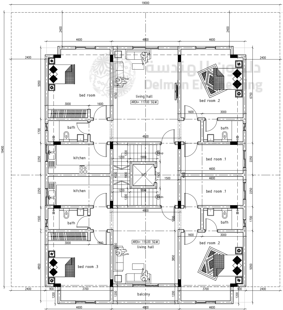
TYPICAL 1st To 5th FLOOR PLAN SCALE 1:100 MTS.
